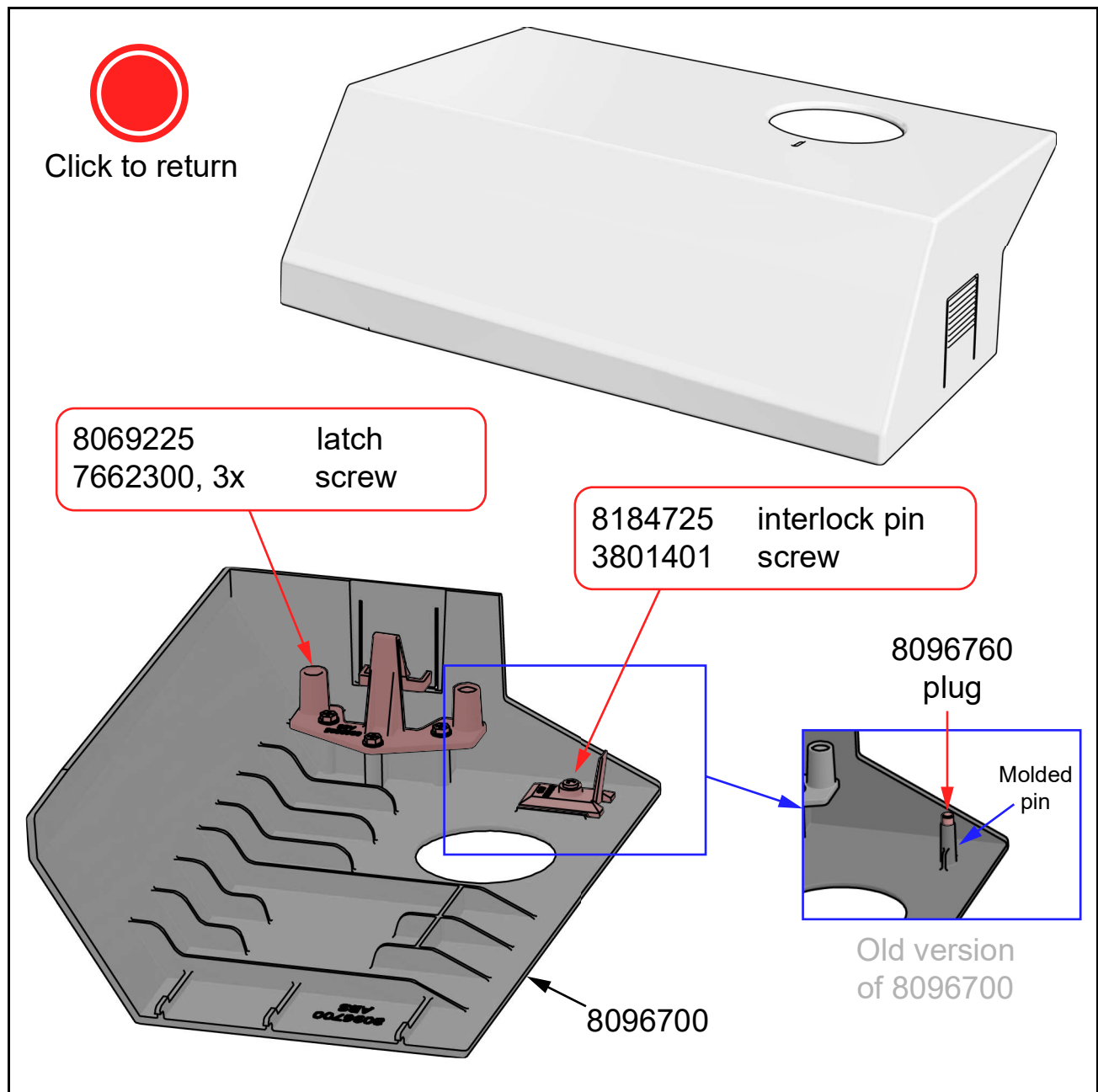
Figure 5-5: 8096700 Transport Cover
